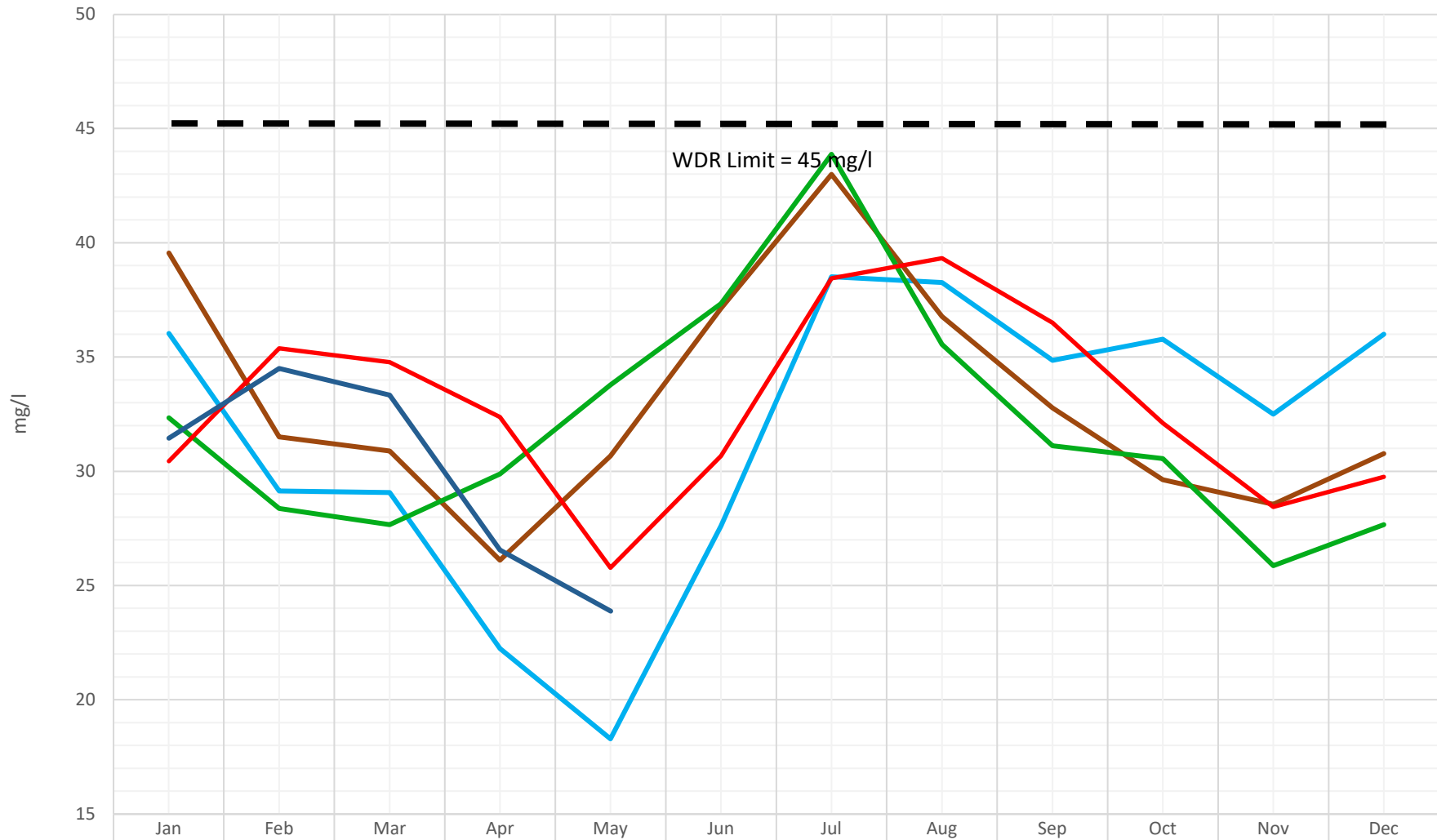
Monthly Average Daily Chemical Oxygen Demand (Effluent)
