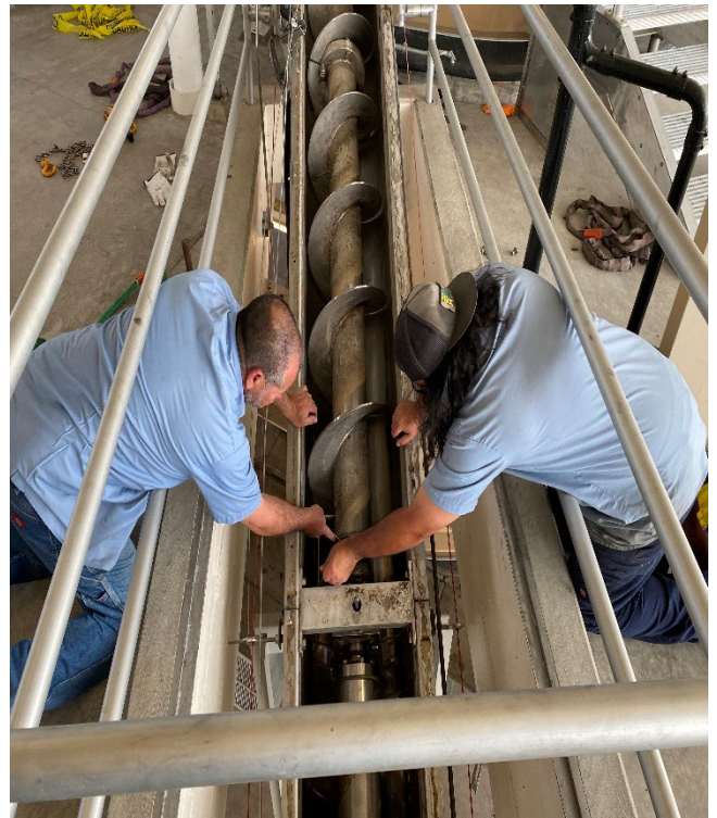
Cake Conveyor Auger
